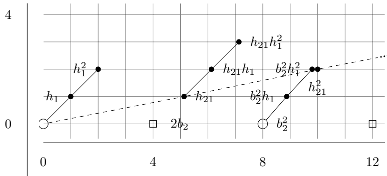
FIGURE 3. The part of the E_4 -page of the spectral sequence which is relevant for b_2 . Although h_{21} h_1^2 appears in this picture, it is only because we have not also drawn in the d_3 -differential on b_4 (which kills h_{21} h_1^2 , as shown in Figure 4).
