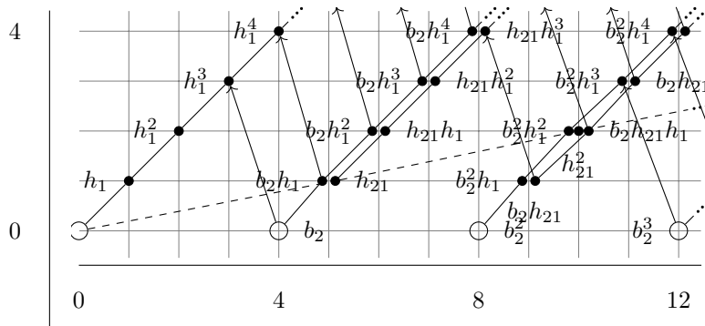
FIGURE 2. Part of the E_3 -page of the spectral sequence, where the “primary” d_3 -differential d_3(b_2) = h_1^3 is indicated. Although it is not hard to extend this drawing further, the spectral sequence starts to look a little cluttered. The sloped lines indicate \eta -multiplication. The dashed line indicates \sigma_1 -multiplication, and we have only indicated it on the unit class to avoid cluttering; we have also not drawn in the classes given by h_1 -multiplies of powers of h_{21} , etc.
