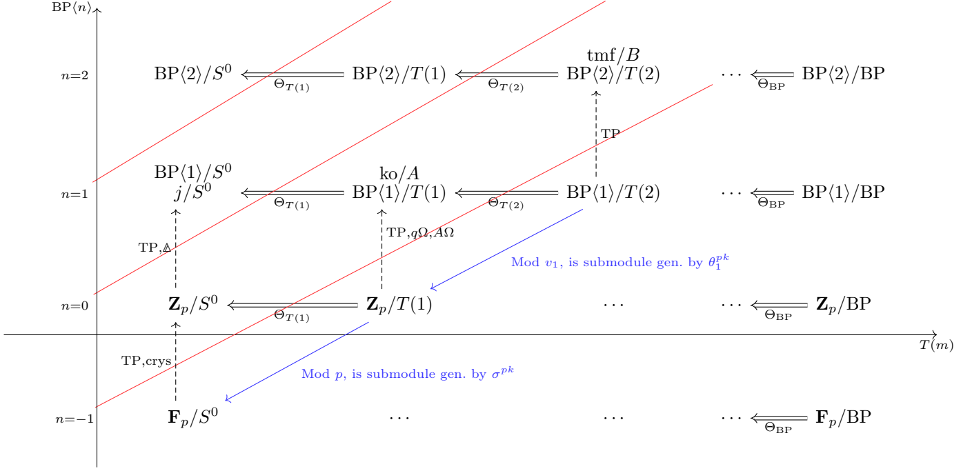
FIGURE 1. Heuristic picture suggested by this article, where we have assumed for simplicity that T\langle m \rangle admits the structure of a framed \mathbf{E}_2 -ring.
